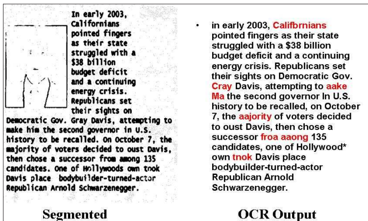
Fig. 24: OCR output: From Binary Image (Using Niblack [2])
